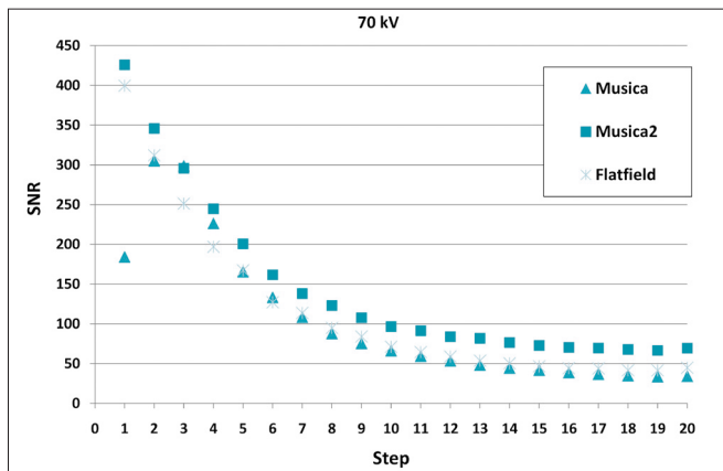
Fig. 2. Signal-to-noise ratios for all steps imaged at 70 kV. Readout artefacts can cause outliers as seen at step 1 (MUSICA).
