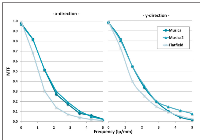
Fig. 5. Modulation transfer functions in both x- and y-axes as calculated on the same MTF plate for all three algorithms. The post-processed images have higher MTF values over all useful frequencies.
