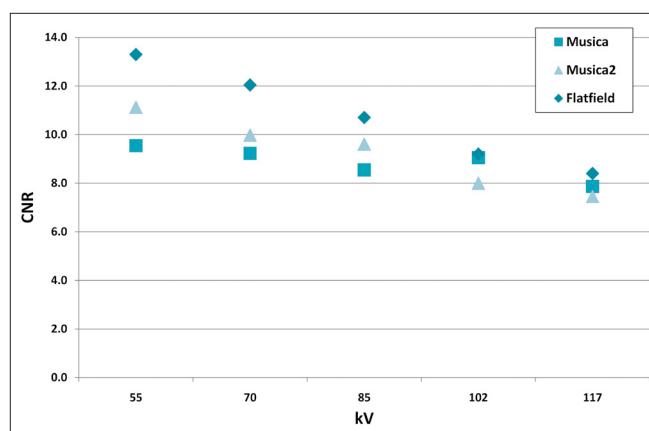
Fig. 3. Average contrast-to-noise ratios calculated from steps 1 to 4 of the step wedge at all energies.
