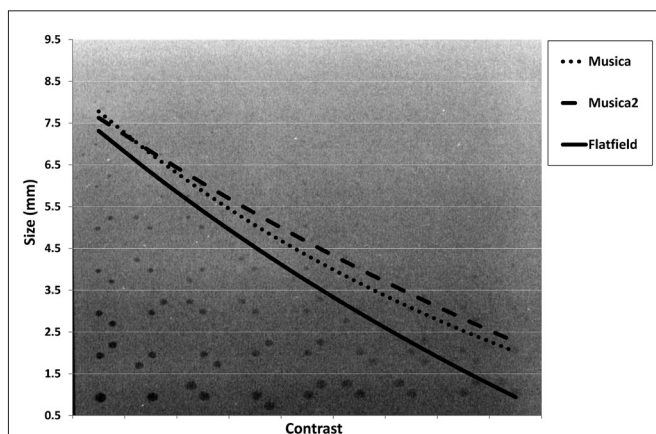
Fig. 4. Graph showing contrast with decreasing object size for the different algorithms.
